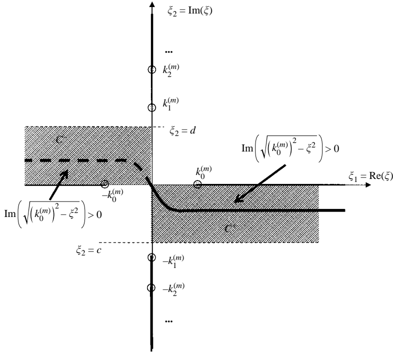
FIGURE 2. The strips S_{c0}^+ and S_{0d}^- and the contour of integration C = C^- \cup C^+ for the Fourier inversion in the complex \xi -domain. The location of the singularities \pm k_0^{(m)}, \pm ik_1^{(m)}, \pm ik_2^{(m)}, \dots , and the associated branch cuts, for each half-strip D^{(m)}, m = 1, 3 , is shown by using small circles and thick lines, respectively. Note that the path of integration is selected to pass through the strips S_{c0}^+ and S_{0d}^- , where \text{Im}(\sqrt{(k_0^{(m)})^2 - \xi^2}) > 0 .
