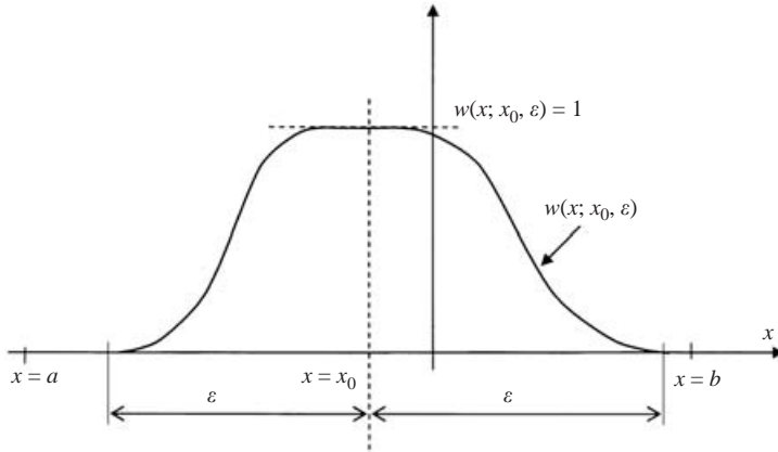
FIGURE 3. The filter function w(x; x_0, \epsilon) = \tilde{w}(|x - x_0|/\epsilon) .
